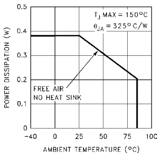
5-Pin Plastic SOT-23 Maximum Power Dissipation vs Ambient Temperature
